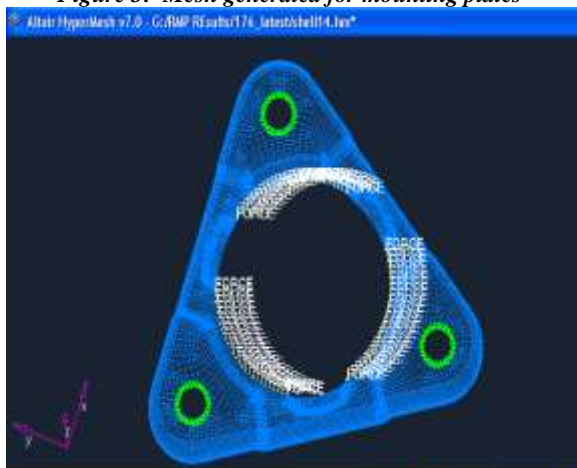
Figure4: Finite element model of the plate with boundary conditions
