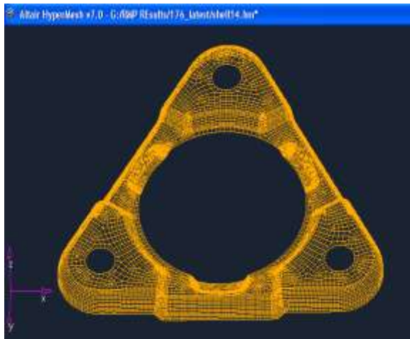
Figure 3: Mesh generated for mounting plates
