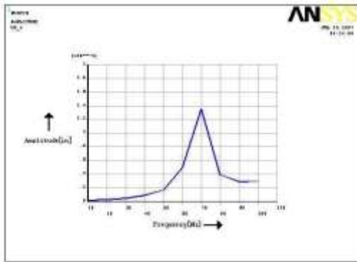
Figure12: Amplitude Vs Frequency at Leg-2
