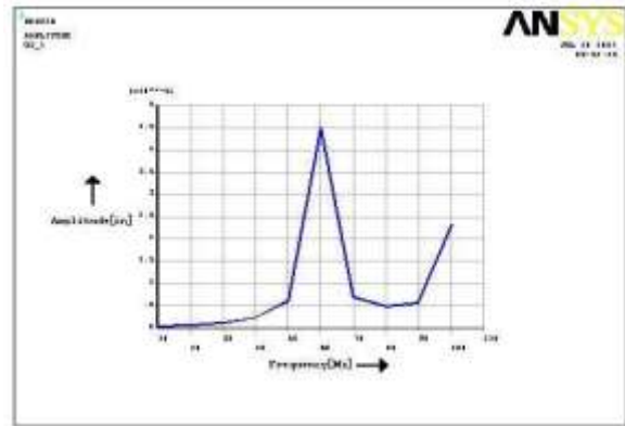
Figure5: Amplitude Vs Frequency at Leg-1
